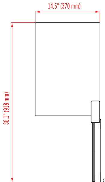
TOP VIEW
